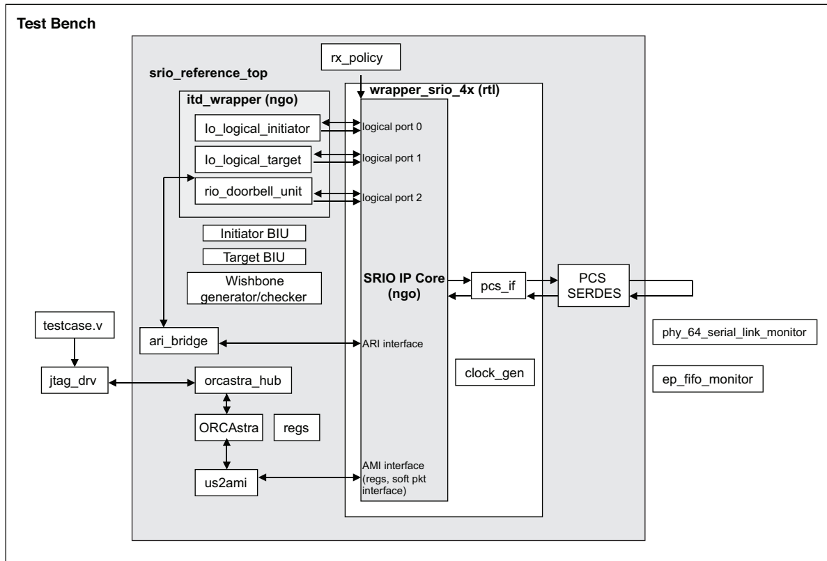
Figure 4-4. Simulation Environment Block Diagram
