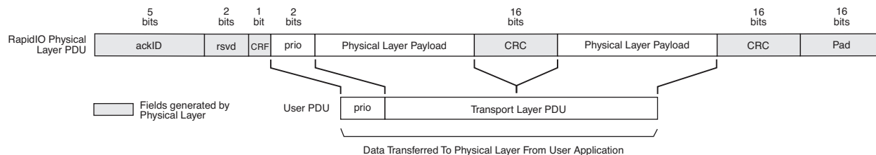
Figure 2-3. Transmit Packet Handling
