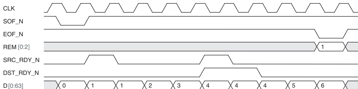
Figure 2-28. Logical Port Data Transfer Diagram With Stalls
