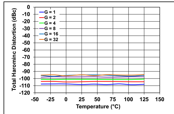
FIGURE 2-5: THD vs. Temperature.
