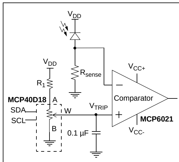
FIGURE 8-2: Set Point or Threshold Calibration.
