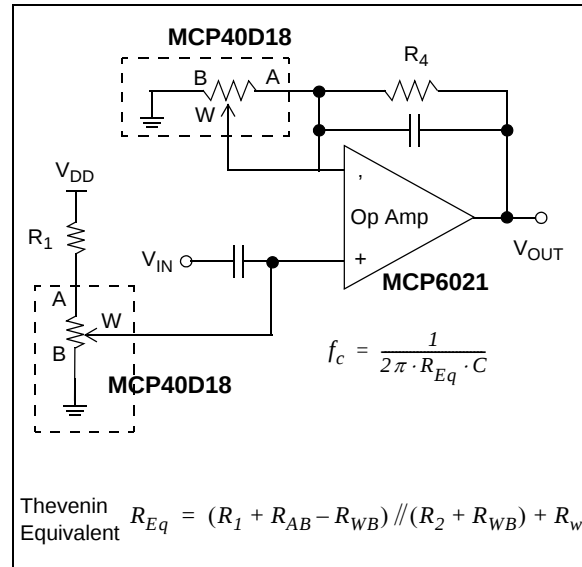
FIGURE 8-4: Programmable Filter.
