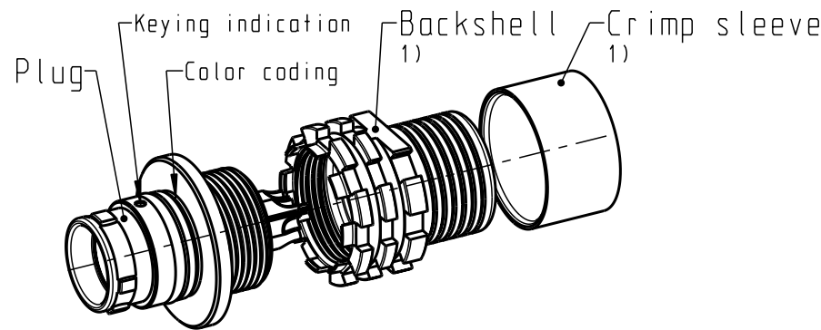
Delivery condition 2:1
