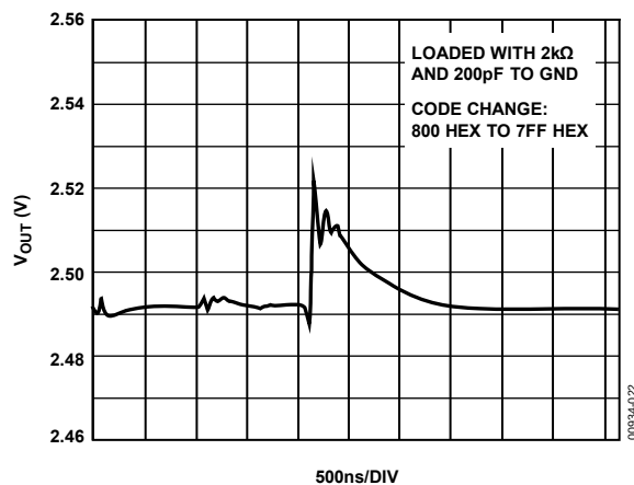
Figure 22. Digital-to-Analog Glitch Impulse
