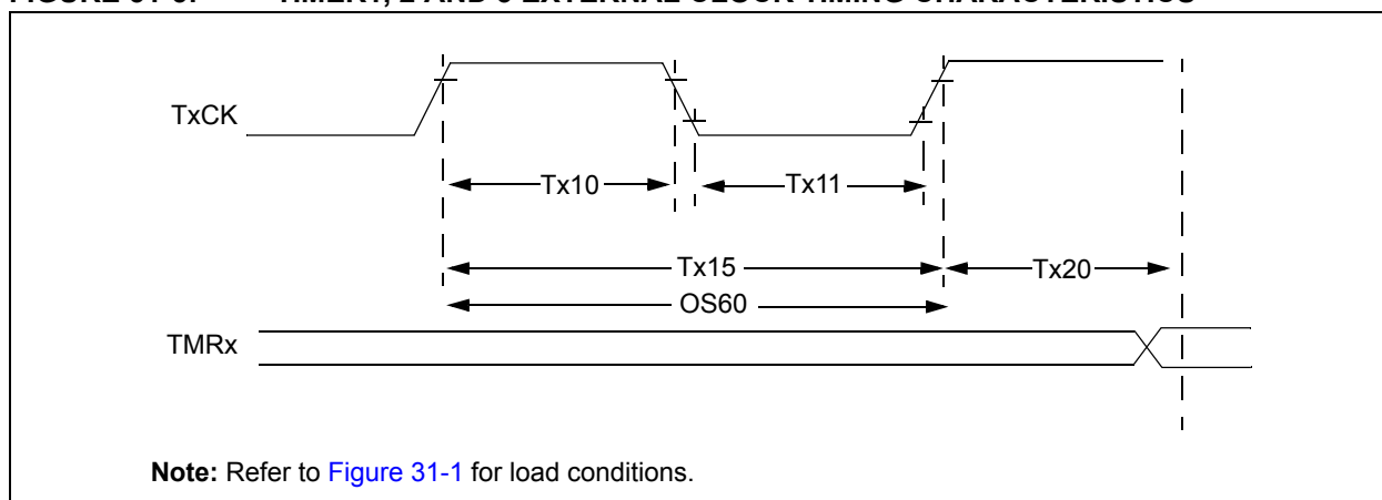
FIGURE 31-5: TIMER1, 2 AND 3 EXTERNAL CLOCK TIMING CHARACTERISTICS
