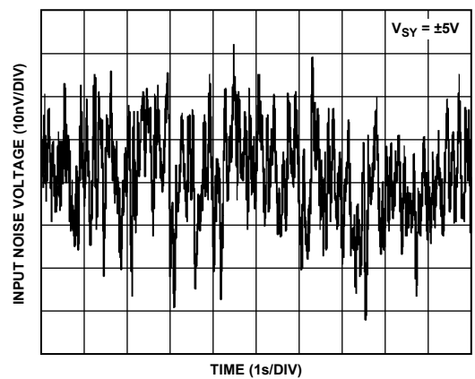
Figure 50. 0.1 Hz to 10 Hz Noise
