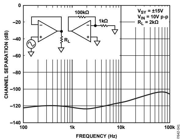
Figure 57. Channel Separation vs. Frequency
