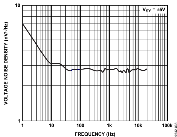
Figure 48. Voltage Noise Density
