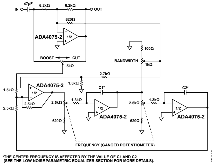
Figure 69. Low Noise Parametric Equalizer
