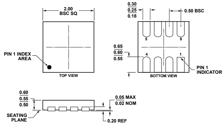
Figure 72. 8-Lead Lead Frame Chip Scale Package [LFCSP_WD]
