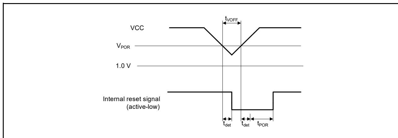
Figure 2.66 Voltage detection reset timing
