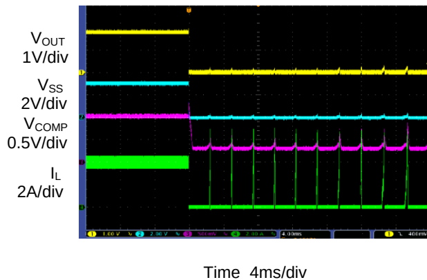
Short Circuit Protection ( V_{IN}=5V , V_{OUT}=1.8V , I_{OUT}=4A )
