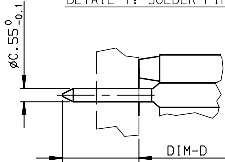
DETAIL-1: SOLDER PIN
