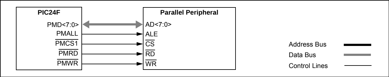
FIGURE 18-10: PARALLEL EEPROM EXAMPLE (UP TO 15-BIT ADDRESS, 8-BIT DATA)
