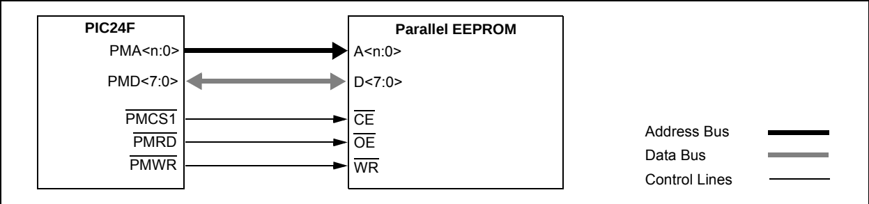
FIGURE 18-11: PARALLEL EEPROM EXAMPLE (UP TO 15-BIT ADDRESS, 16-BIT DATA)
