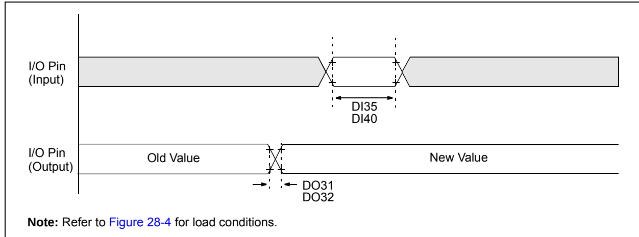
FIGURE 28-6: CLK0 AND I/O TIMING CHARACTERISTICS
