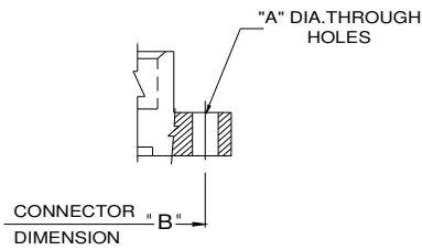
MOUNTING OPTION CODES x102 AND x104 (THROUGH MOUNTING HOLES)
