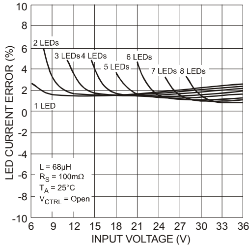
Figure 21. LED Current Deviation vs. Input Voltage
