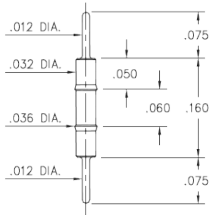
9075-0-00-XX-00-00-03-0 Press-fit in .034 mounting hole
