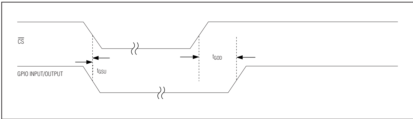
Figure 13. GPIO Timing
