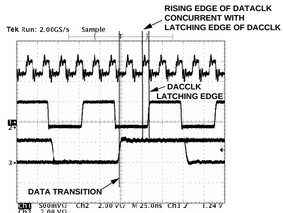
Figure 56. DATAADJ = 0001
